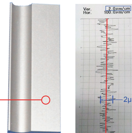
wire mark is 2 \mu m after 3 cuts
