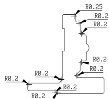
The complex stamping mold has fine 3 \mu m tolerance with average 1mm height of cutting edge.
