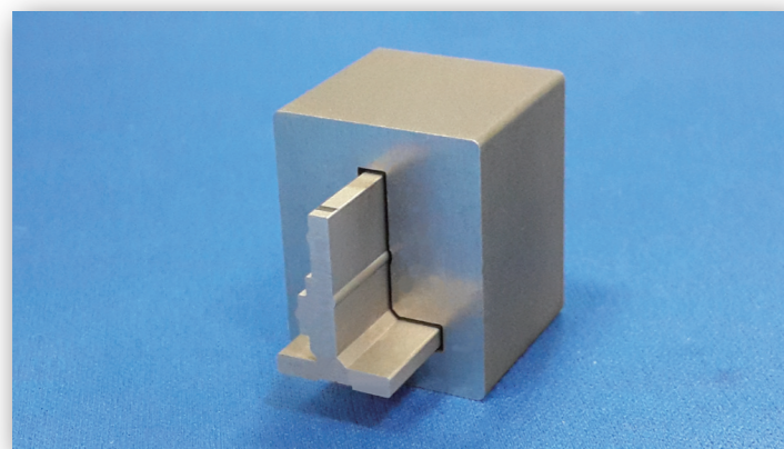
The complex stamping mold has fine 3 \mu m tolerance with average 1mm height of cutting edge.
